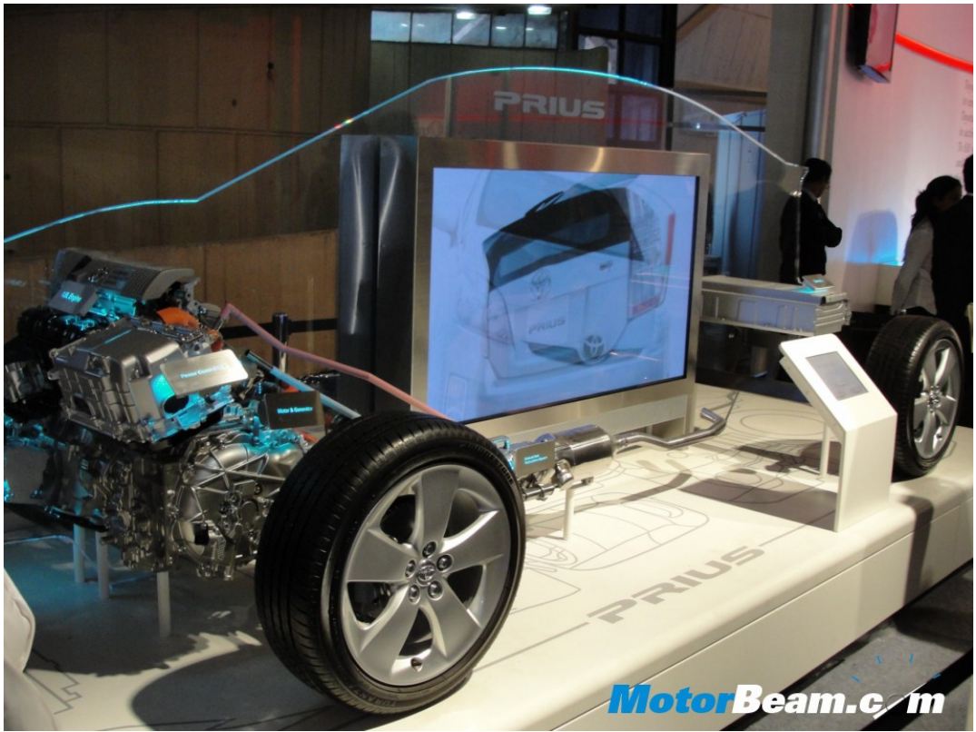
Toyota Hybrid Synergy Drive System II :-
